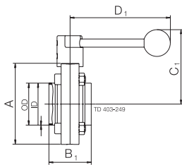
a. LKB Low Pressure with welding ends.
