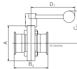
b. LKB Low Pressure with clamp ends.
